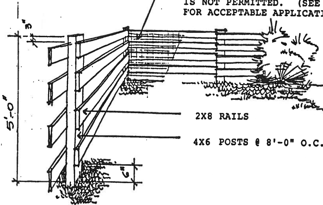
5'-0" HIGH 4 RAIL FENCE TYPE B
