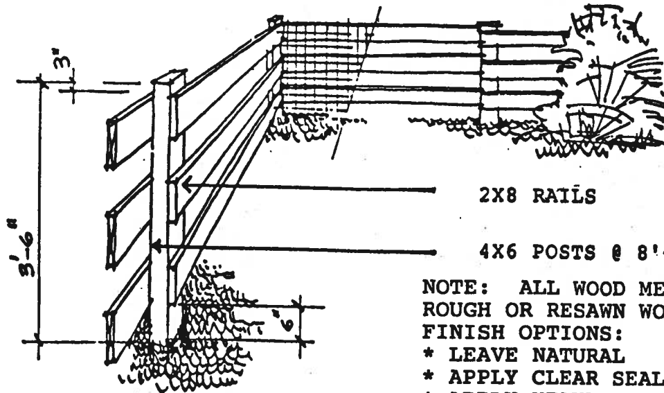
3'-6" HIGH 3 RAIL FENCE TYPE A
