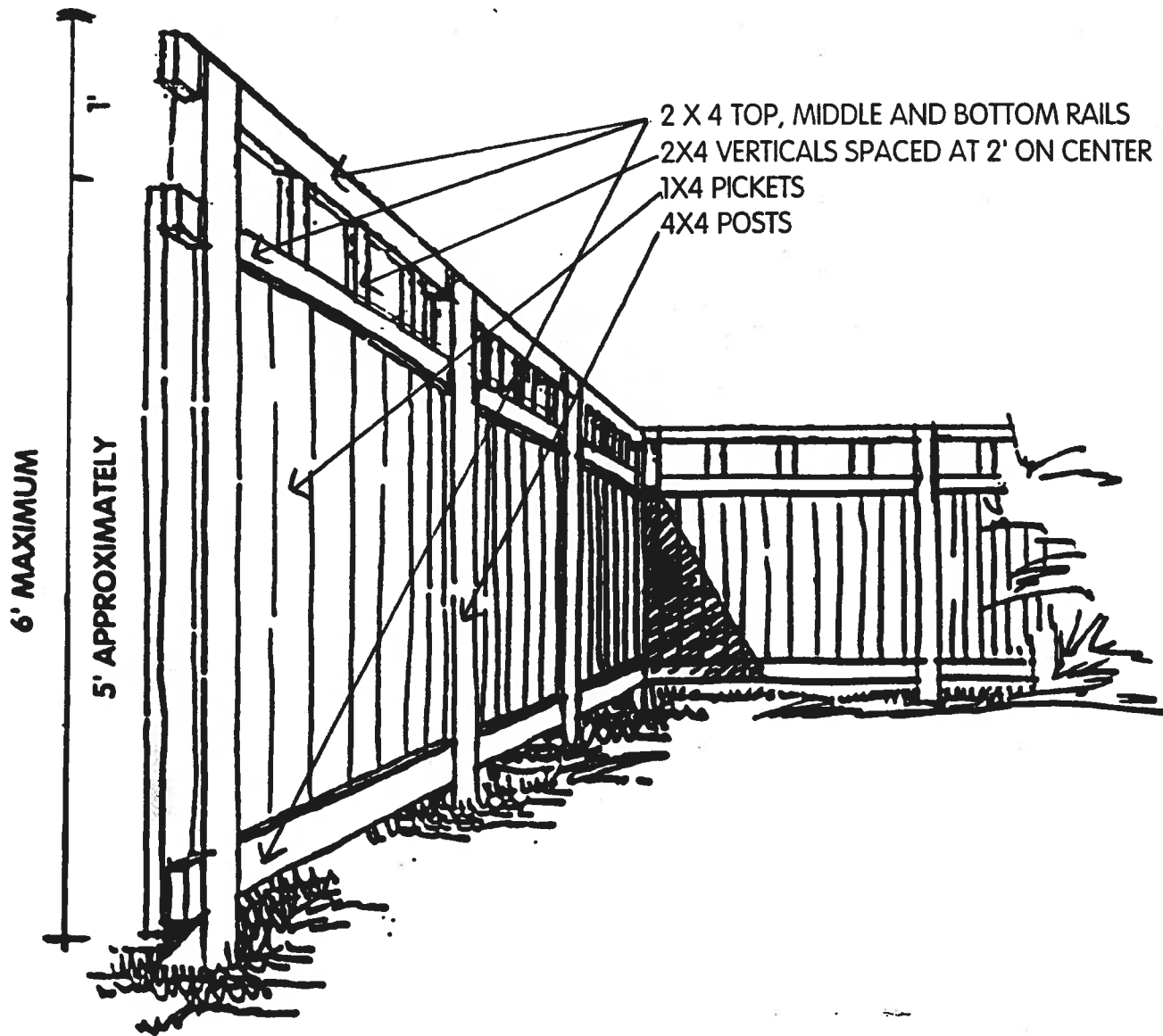
ORIGINAL PRIVACY OPAQUE FENCE DESIGN TYPE E
